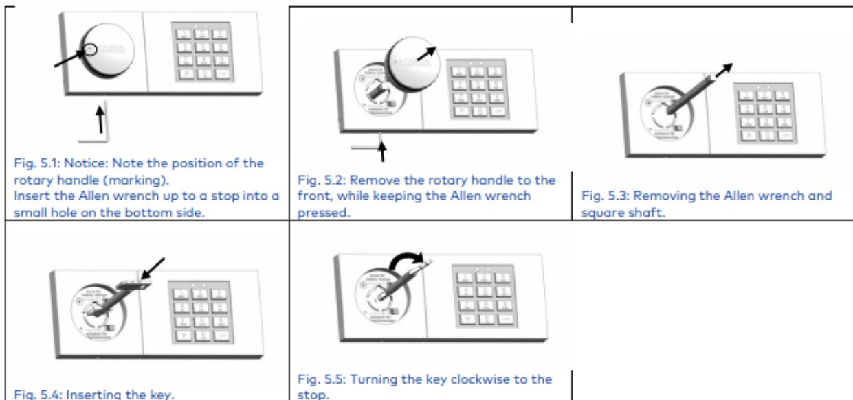
Figure 5: Opening with the key
