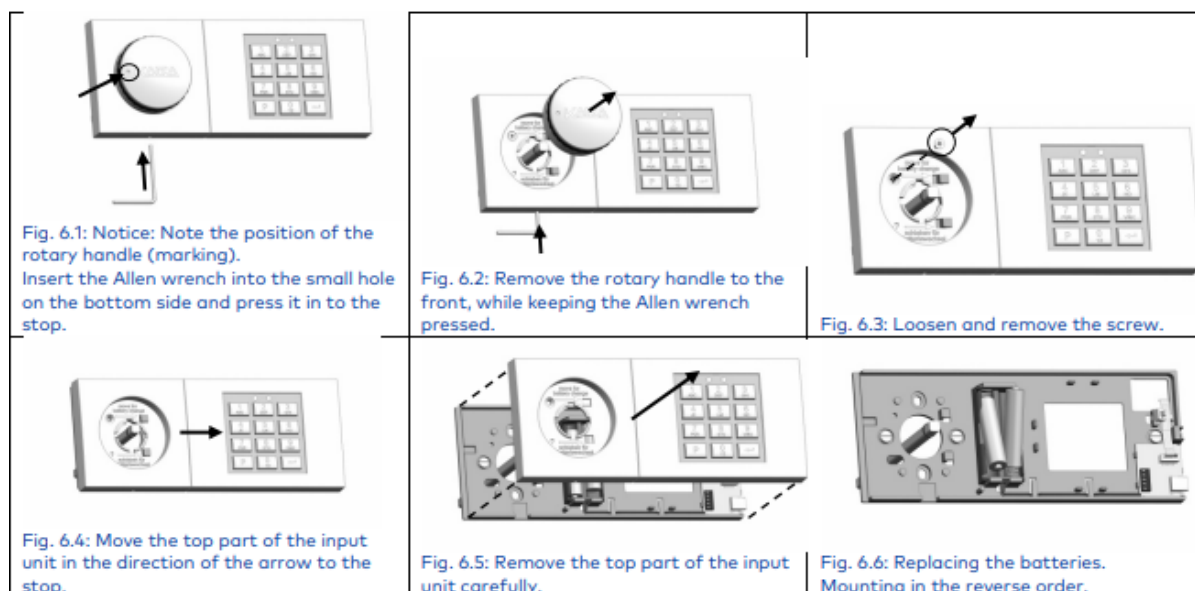
Figure 6: Battery replacement
