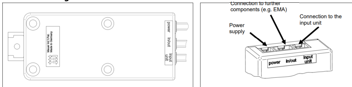
Figure 3: Lock housing
